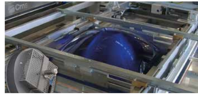
Sheet bubble electronic system: the bubble function is created using an electronically controlled fan. The bubble height control is achieved with the laser, infra-red or ultrasound sensor.
