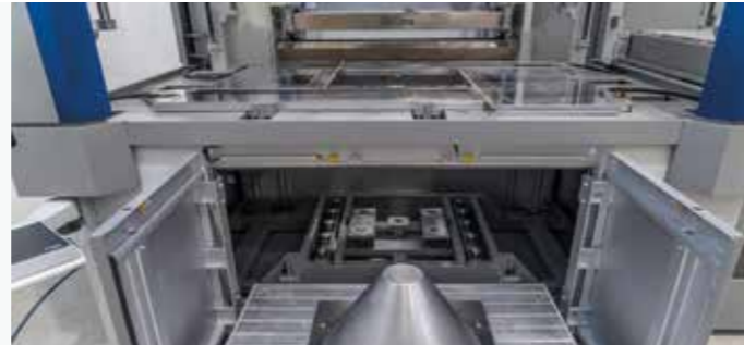
Quick mould change: removable mould plate with its own cart. The cart can be fitted with mould lifting device for the utmost in terms of production change speed. Simplifies the centring operations and equipment installation on the outside of the machine.
