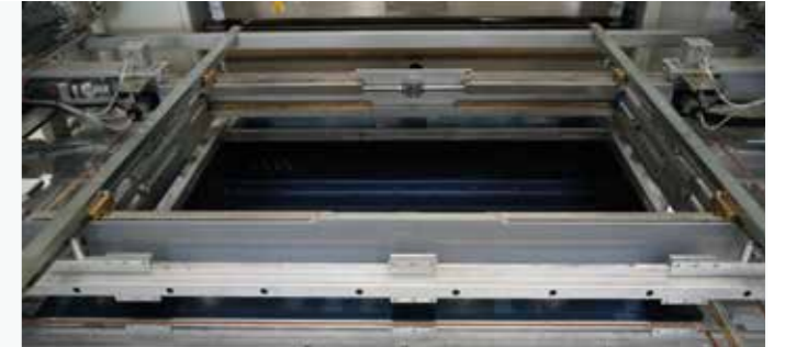
Automatic reduction plate: diaphragm system to adapt the machine dimension to the mould by reducing scrap material to a minimum without the need for specific equipment
