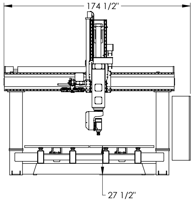
10'(w) x 5'(d) x 48"(h) Moving Table (pictured)
